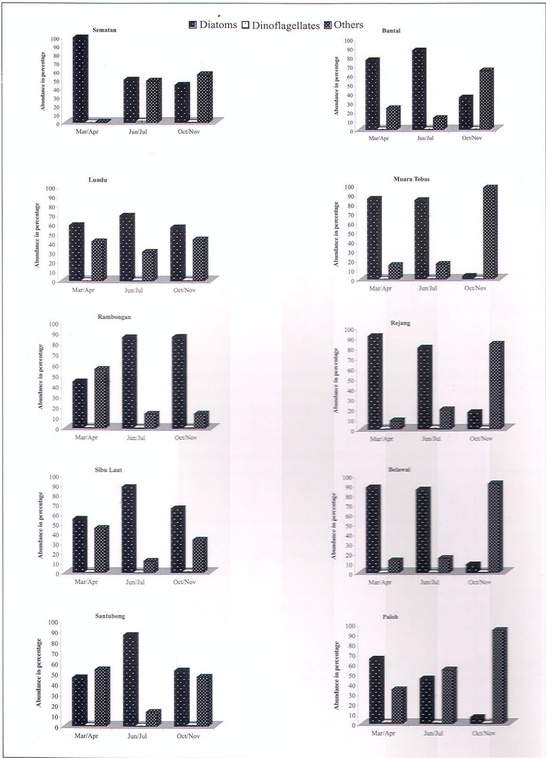
Figure 1: Phytoplankton abundance for diatoms, dinoflagellates and others in percentage on three sampling periods at 10 locations
