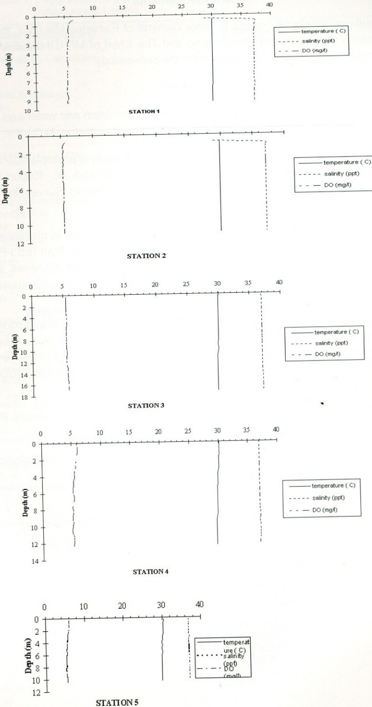
Figure 4: The value of temperature, Salinity and DO inside the lagoon of Pulau Layang Layang at various stations and water depth
