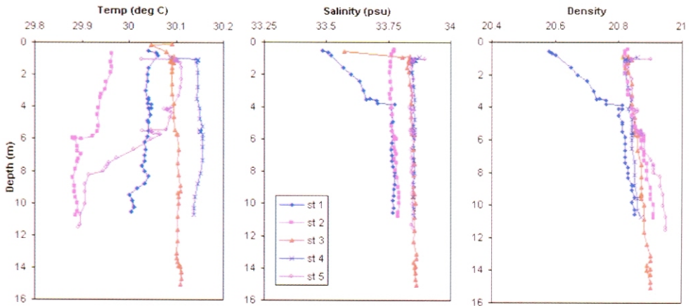
Figure 9: Temperature, salinity and density profiles in the lagoon
