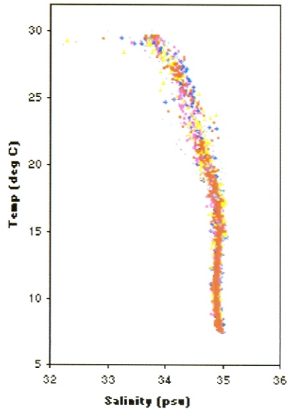
Figure 8: The T-S diagram of all the stations of Pulau Layang Layang.
